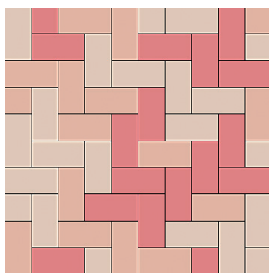
B-1 + B-2 + R-2 16.7個/㎡ + 16.7個/㎡ + 16.7個/㎡
