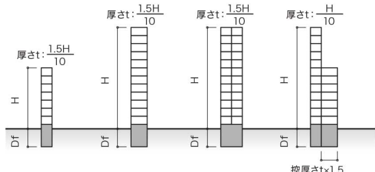
図2-3-1 組積造の塀断面例
